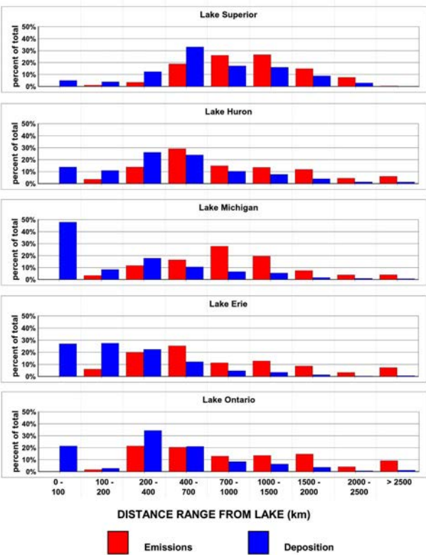
FIGURE 20 Percent of Total Estimated Emissions and Model-estimated Deposition of Mercury to the Great Lakes Contributed from Different Distance Ranges Away from Each Lake
