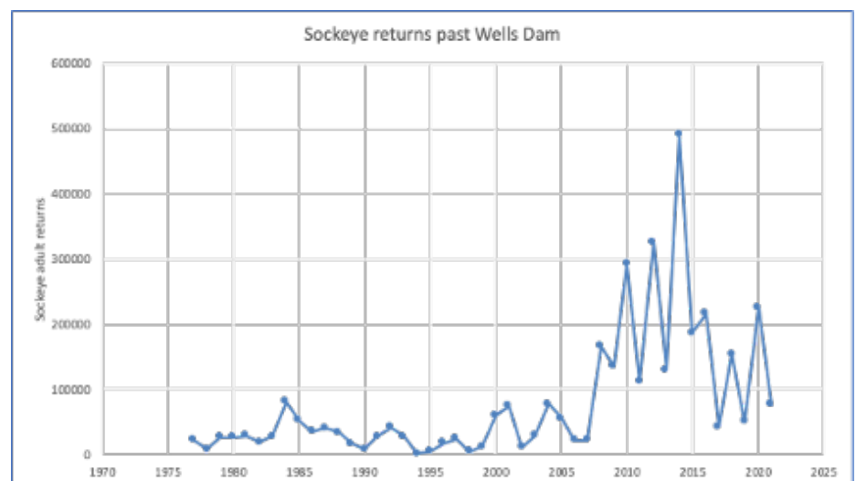
Figure 7. Historic Sockeye Salmon returns at Wells Dam. Wells Dam is located just downstream of the confluence of the Okanagan and Columbia Rivers.
