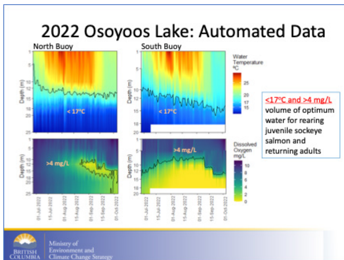
Figure 10. Osoyoos Lake water column temperature and dissolved oxygen trends for Summer 2022. Juvenile sockeye salmon optimal rearing habitat requires <17c and >4 mg/L dissolved oxygen, which significantly limits habitat area to the north basin (buoy) which is 'squeezed' to near zero optimum habitat in late summer. Source: BC Ministry of Environment and Climate Change Strategy.
